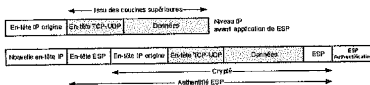
Figure 24.27 Authentification ESP en mode tunnel
