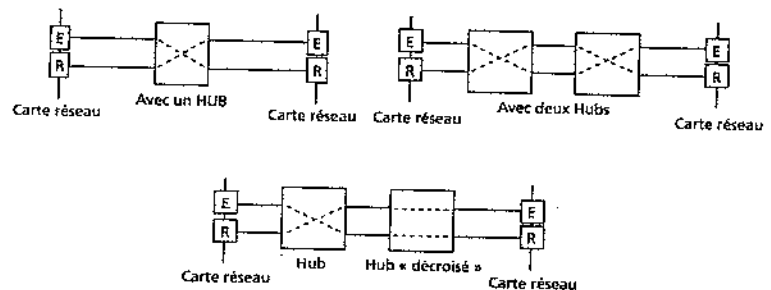
Figure 26.5 Cascade de Hubs
