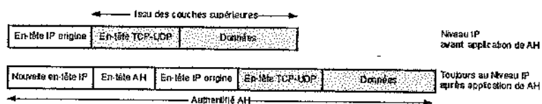
Figure 24.25 Authentification AH en mode tunnel
