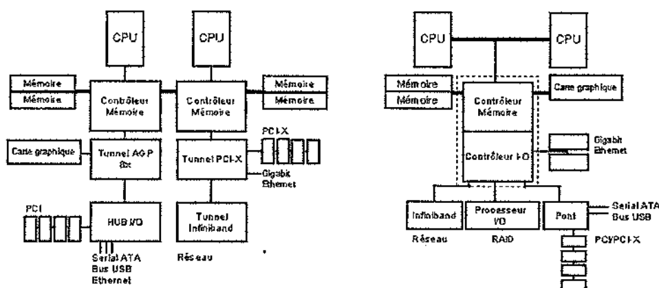
Figure 9.6 HyperTransport - PCI-Express
