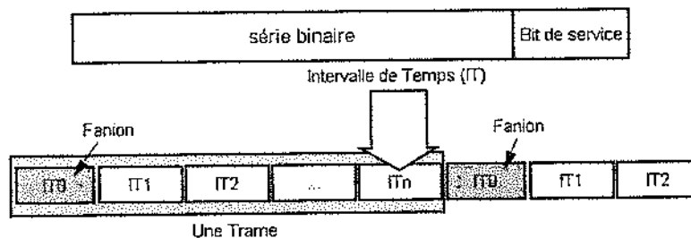
Figure 21.12 Multiplexage temporel fixe
