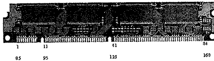
Figure 11.15 Barrette au format DIMM 168 broches
