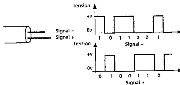
Figure 2.3 Transmission symétrique
