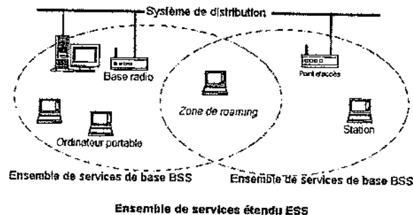
Figure 22.17 Mode infrastructure
