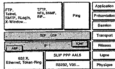
Figure 24.22 La pile TCP/IP
