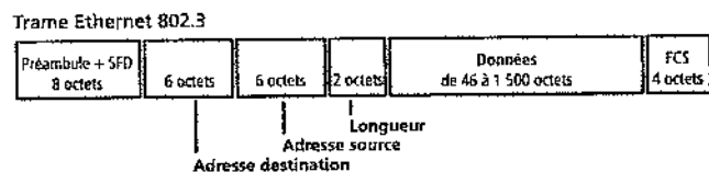
Figure 25.5 Trame Ethernet 802.2
