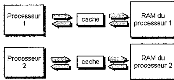
Figure 10.11 Architecture parallèle
