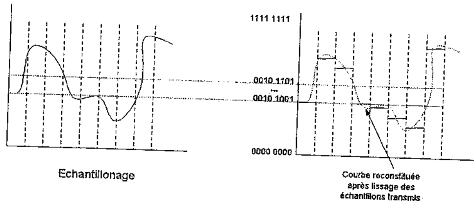
Figure 21.9 Modulation MIC
