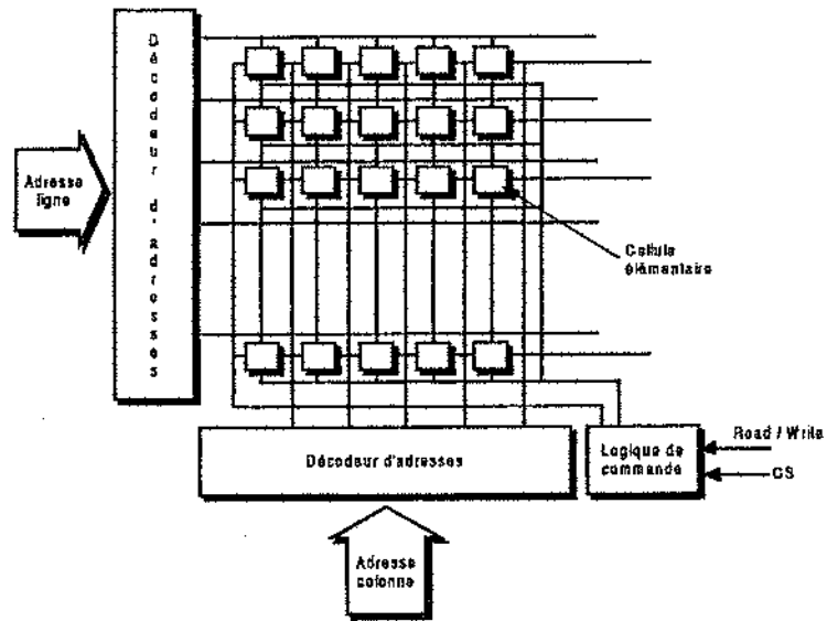
Figure 11.8 Organisation de la mémoire FPM
