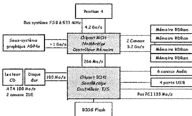
Figure 10.4 Structure d'un chipset
