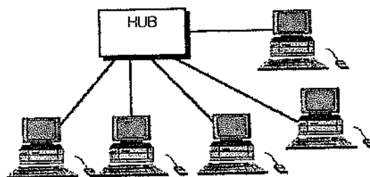
Figure 22.1 Topologie étoile
