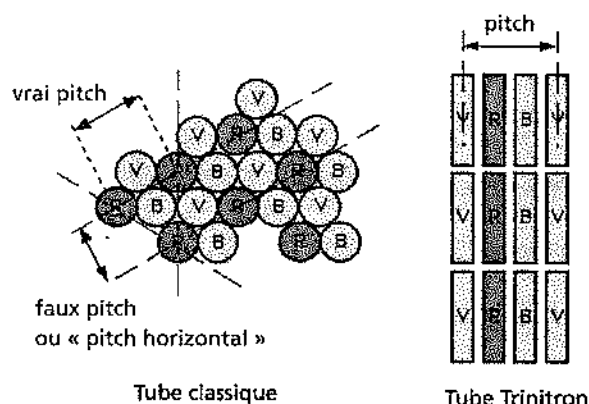
Figure 19.2 Le pitch
