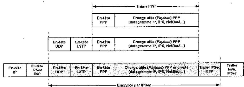
Figure 26.20 Encapsulation IPSEC et L2TP
