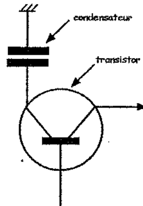
Figure 11.4 Cellule mémoire DRAM
