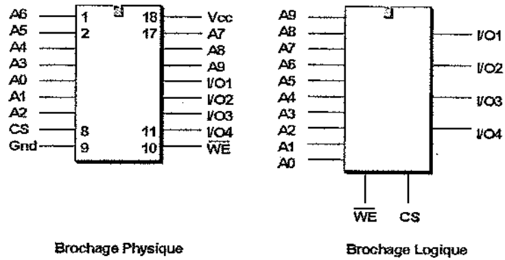
Figure 11.9 Brochage mémoire
