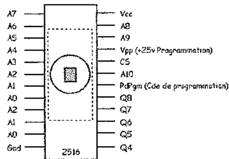
Figure 11.18 Mémoire EPROM
