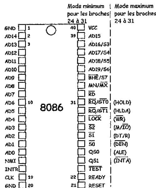
Figure 10.1 Brochage du 8086
