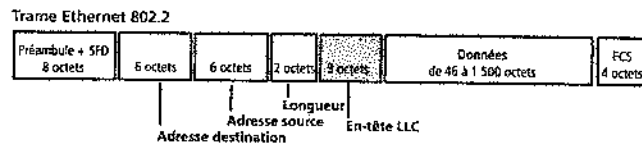
Figure 25.6 Trame Ethernet SNAP
