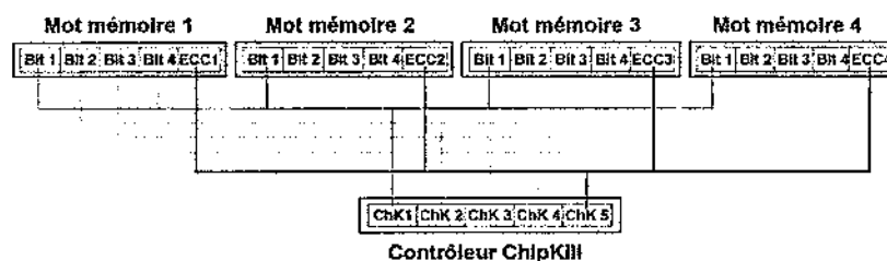
Figure 11.7 Mémoire ChipKill ECC
