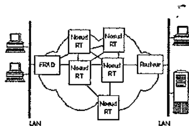
Figure 23.13 Architecture du relais de trames
