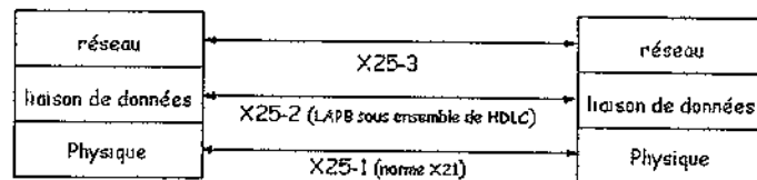
Figure 23.7 La norme X25
