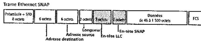
Figure 25.7 Trame Ethernet 802.3
