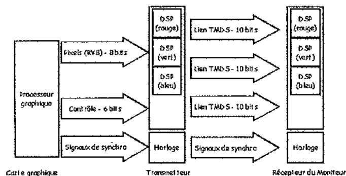
Figure 19.3 Interface DVI
