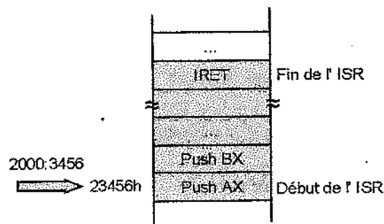
Figure 8.8 L'ISR ( Interrupt Service Routine )
