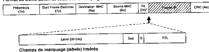
Figure 26.21 Trame MPLS
