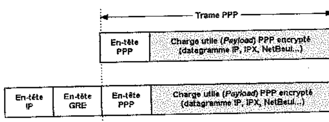
Figure 26.19 Trame PPTP
