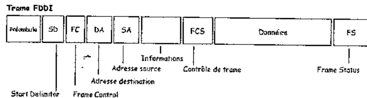
Figure 26.15 Trame FDDI
