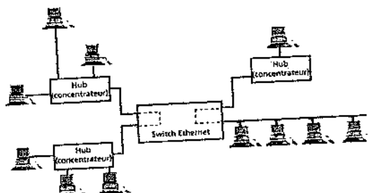
Figure 26.8 Commutation de segments
