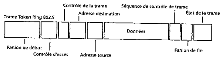
Figure 25.16 Trame Token Ring 802-5
