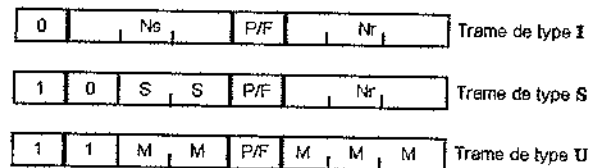
Figure 23.5 Types de trames
