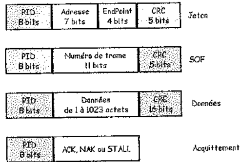
Figure 9.10 Types de paquets USB
