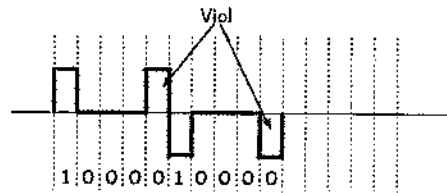
Figure 5.11 Encodage HDB3
