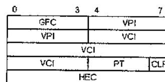
Figure 23.16 En-tête UNI
