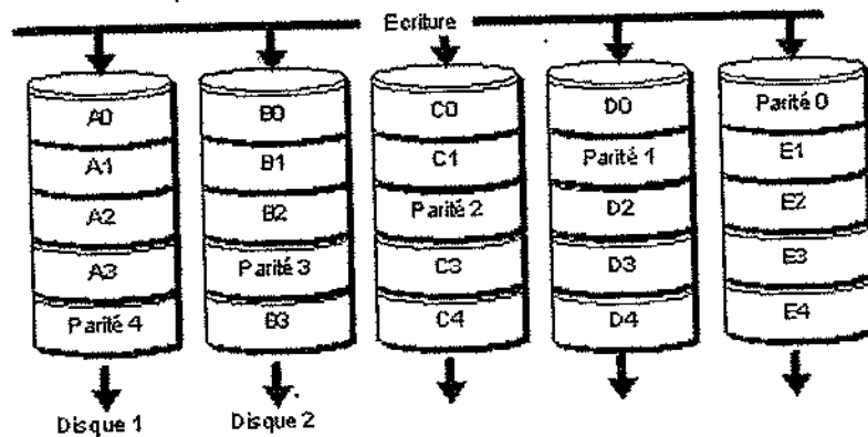
Figure 13.11 RAID-5
