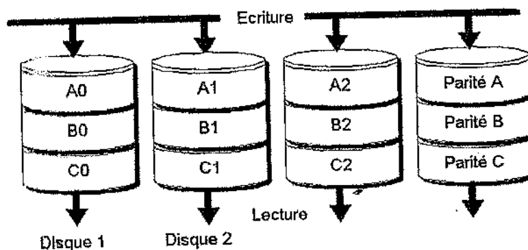
Figure 13.10 RAID-3
