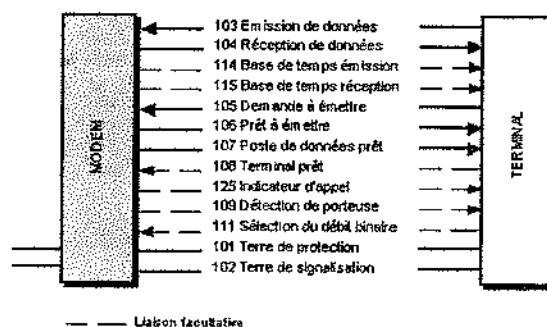
Figure 22.8 Connexion DB25
