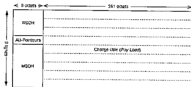
Figure 23.19 Structure de la trame STM-1
