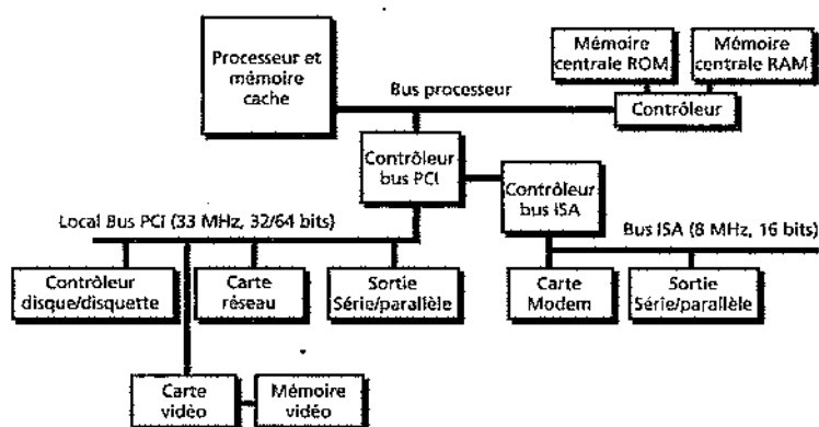
Figure 9.5 Architecture du bus PCI
