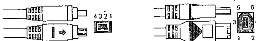
Figure 9.8 FireWire 4 pins et 6 pins
