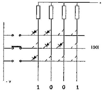
Figure 11.16 Matrice mémoire
