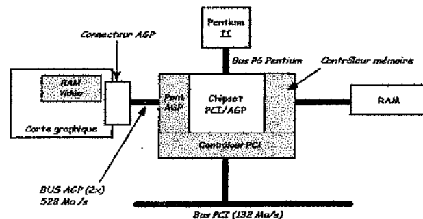
Figure 9.11 Le bus AGP 2x
